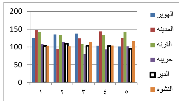
Figure (31) of the enrichment factor (Pb) wet season
