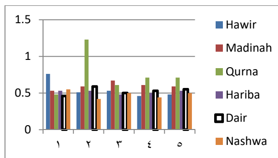
Figure (38) of the Contamination factor (cu) dry season
