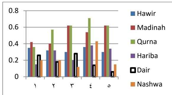
Figure(18)value (I-geo) (cu) dry season
