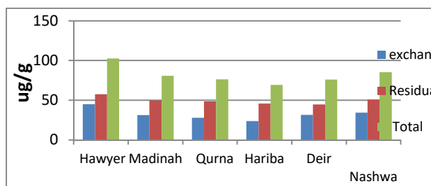
Figure (10) Concentrations of Nickel (ug/g) dry season
