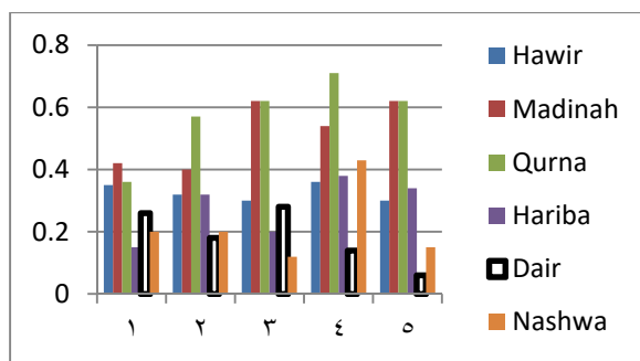
Figure (39) of the Contamination factor (cu) wet season
