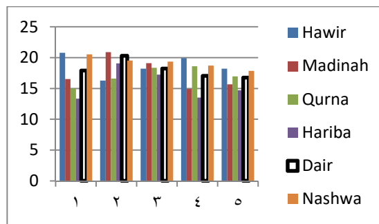
Figure (25) value (I-geo) (cd) wet season
