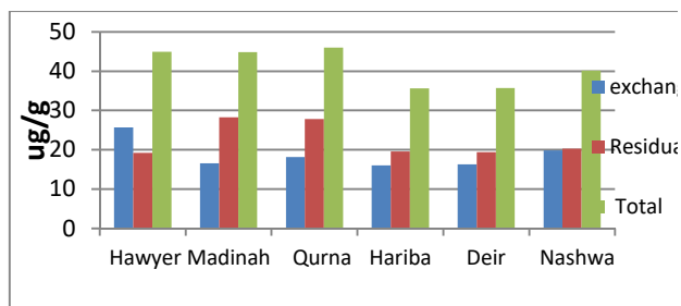
Figure (9) Concentrations of Lead (ug/g) wet season
