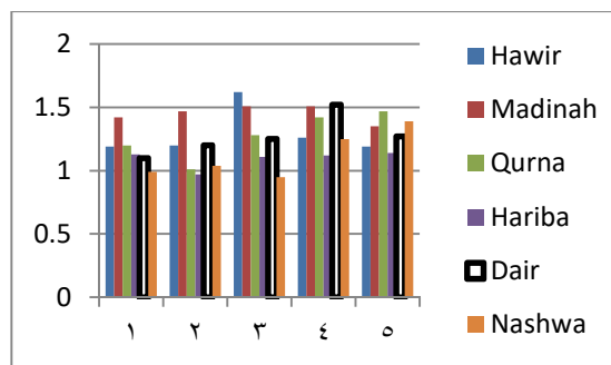
Figure (37) of the Contamination factor (Zn) wet season
