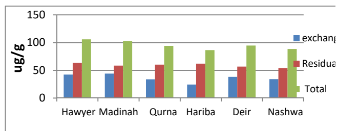
Figure (11) Concentrations of Nickel (ug/g) wet season
