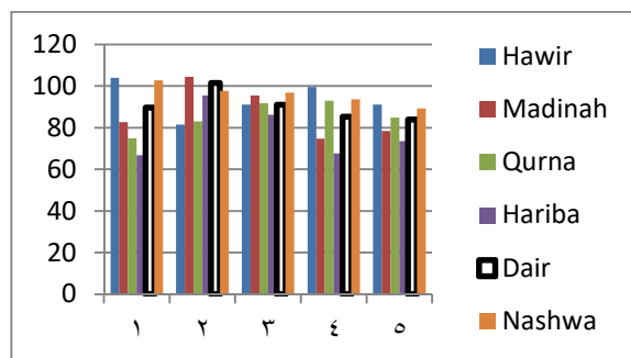
Figure(45) of the Contamination factor (cd) wet season
